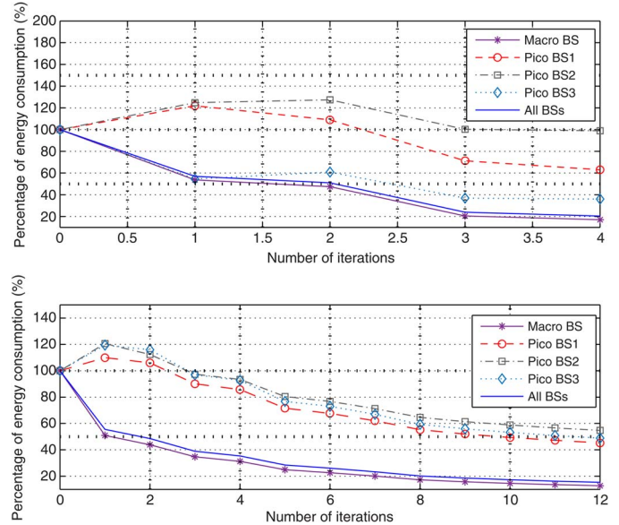
Fig. 7. Power consumption with different convergence precision. Upper: \Delta_1 = 10^{-1} ; Lower: \Delta_1 = 10^{-2} .
