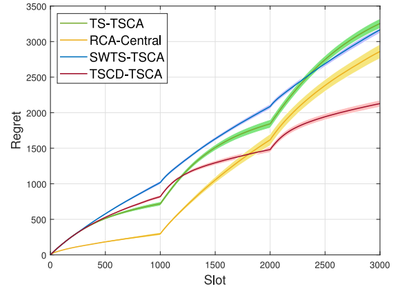
(a) Non-stationary Bernoulli model
