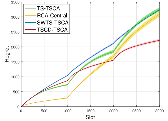
(b) Non-stationary Markovian model
